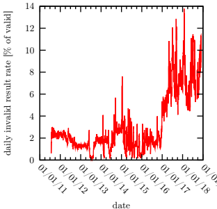
Daily Invalid Result Rate for BRP4
