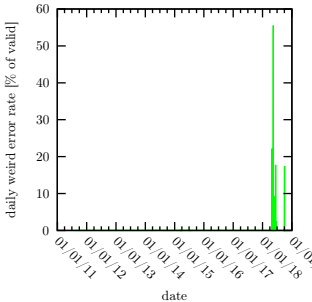
Daily Weird Error Rate for BRP4
